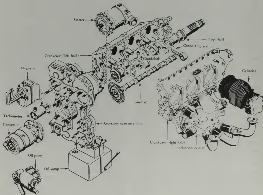
FIGURE 1-7. Typical opposed engine exploded into component assemblies.
